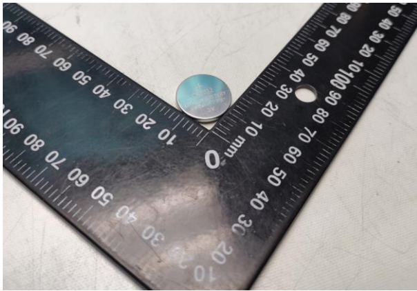
Cell/电芯 (CR2032 3,0V 210mAh)
