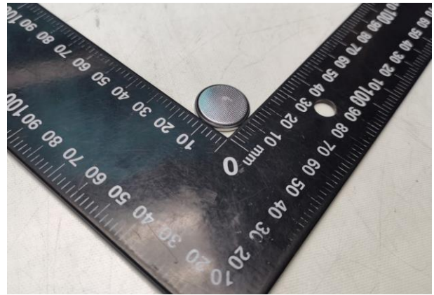
Cell/电芯 (CR2032 3,0V 210mAh)
